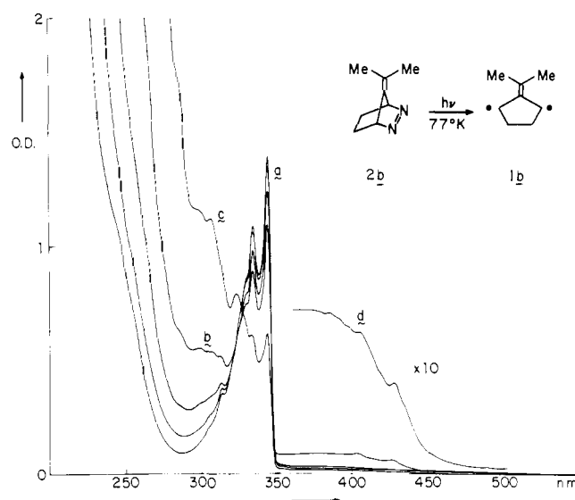
Figure 2. UV/vis spectra recorded during stepwise photolysis of 2b in EPA at 79 K, concn (300 K) 7.8 \times 10^{-2} M (a) before irradiation. (b) same after 10 min exposure ( 320 \text{ nm} < \lambda < 380 \text{ nm} ). (c) same after 33 min exposure. (d) same after 47 min exposure (expanded 10 \times ).
