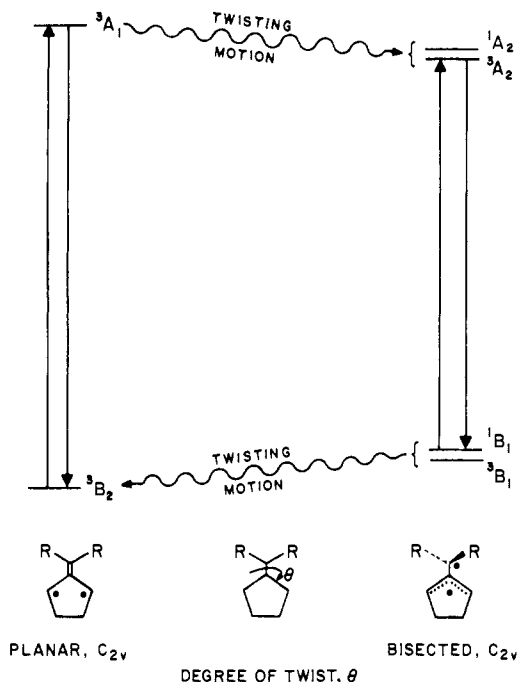
Figure 4. Schematic diagram of the interconversion of trimethylmethane species. Planar and bisected geometries are shown as specific possibilities.
