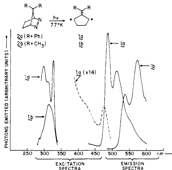
Figure 3. Emission and excitation spectra of irradiated solutions of 2a and 2b at 77 K in MCH. All intensities are arbitrary and do not reflect relative emission efficiencies. All spectra are corrected for instrumental response varying with wavelength. The dotted curve labeled 1a ( \times 14 ) is the excitation spectrum of 1a in the longer wavelength region at 14 times the sensitivity of the excitation spectrum of 1a at shorter wavelength.
