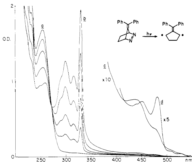
Figure 1. UV/vis spectra recorded during stepwise photolysis of 2a at 79 K (a) before photolysis (Initial concentration in MCH at 300 K: 1.1 \times 10^{-3} M). (b) same after a total of 290 s exposure ( \lambda 254 nm) (Intermediate spectra shown). (c) same after 560 s exposure (expanded 10 \times ). (d) spectrum (expanded 5 \times ) after 86 min photolysis of a 1.1 \times 10^{-2} M solution of 2a in EPA.
